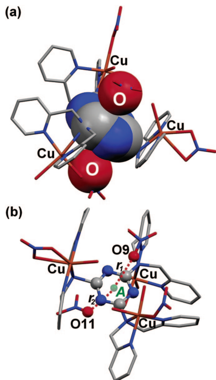
FIGURE 9. (a) Representation of the cation [\text{Cu}_3(\text{dipictriaz})-(\text{NO}_3)_2(\text{H}_2\text{O})_6]^{4+} showing the nitrate...triazine...nitrate interactions. 43 (b) Distances between the triazine centroid A and the oxygen atoms O9 and O11 of two free nitrates, r_1 = 3.201 \text{ \AA} and r_2 = 3.502 \text{ \AA} , respectively.
