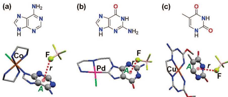
FIGURE 17. Attractive contacts with DNA bases. (a) Tetrafluoroborate–adenine interaction; distance of F \cdots centroid A, r = 3.271 Å [Cambridge Structural Database (CSD) code ICIDII]. (b) Tetrafluoroborate–guanine interaction; r = 3.241 Å (CSD code IBIDIG). (c) Tetrafluoroborate–thymine interaction; r = 3.282 Å (CSD code IVOROA).
