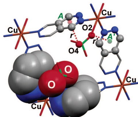
FIGURE 14. Two-dimensional coordination network (square grid) formed by the complex [\text{Cu}(\text{H}_2\text{O})_2(\text{L})_2](\text{ClO}_4)_2 \cdot n\text{H}_2\text{O} ( L = \text{pyridazino}[4,5-d]\text{pyridazine} ), showing the incorporation of two perchlorate anions inside a square cage. 46 Distance between the oxygen atom O4 of the perchlorate anion and the pyridazine centroid A , r = 3.051 \text{ \AA} ; distance between the oxygen atom O2 of the perchlorate anion and the pyridazine centroid A , r' = 3.497 \text{ \AA} .
