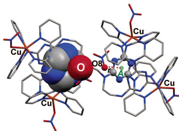
FIGURE 11. Representation of the cation [\text{Cu}_4(\text{dpatta})(\text{NO}_3)_4]^{4+} showing the nitrate...triazine interactions. 45 The separation between the nitrate oxygen atom O8 and the centroid A of the triazine ring is r = 3.230 \text{ \AA} .
